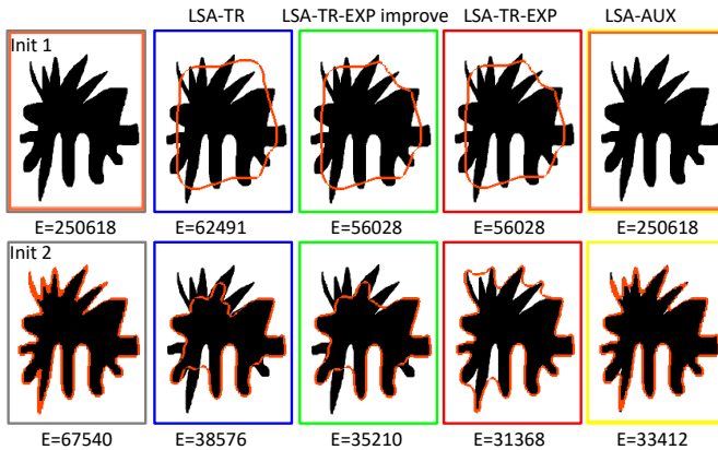
Fig. 14. Local optimization of squared curvature might yield different segmentation results for different initializations. First row - starting with all pixels assigned to foreground, second row - starting with appearance based ML labeling. Here we used \lambda_{\text{curv}} = 1000 .
