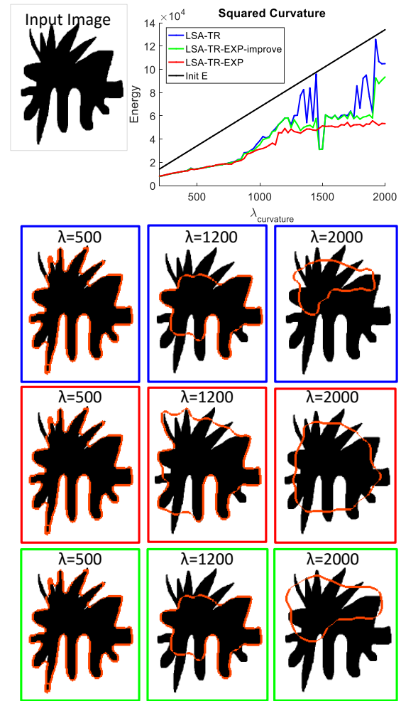
Fig. 13. Optimization of squared curvature model. Top-left: input image with one foreground object. Top-right: Comparison of optimization energies as a function of increasing curvature weight \lambda_{curv} . LSA-TR (blue line) optimizes the energy starting from the maximum likelihood solution based on appearance terms. We used normal distribution \mathcal{N}(\mu, \sigma^2) with (\mu = 0, \sigma = 0.2) for the foreground and (\mu = 1, \sigma = 0.2) for the background respectively. We used 7 \times 7 neighborhood for the angular resolution. LSA-TR-EXP-improve (green line) attempts to improve the final solution of LSA-TR using expansion moves. LSA-TR-EXP (red line) performs expansion moves starting from the same initial solution as LSA-TR. The energy of the initial solution is shown in black. In the bottom of the figure we show final solution of the three methods for three different values of \lambda_{curv} . Blue, red and green frames correspond to results of LSA-TR, LSA-TR-EXP and LSA-TR-EXP-improve respectively.
