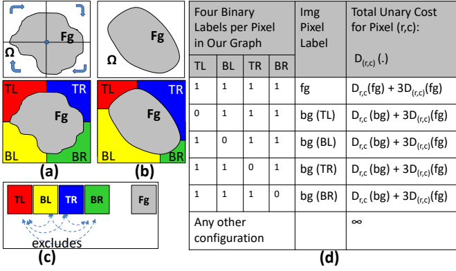
Fig. 10. Compact Shape Prior Illustration: (a-top) the model in [33], (a-bottom) our multilabel model, (b-top) - an input silhouette that can be modeled with our model but not with the model in [33] (see text for details), (b-bottom) demonstrates how we split the image into five regions in our new model, (c) schematic representation of the geometric exclusion constraints between the layers of our graph for our model. (d) unary terms for each layer used in our graph
