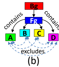
Fig. 8. Multi-part object model for liver segmentation: (a) schematic representation of the liver containing four distinct and mutually excluding tumors. (b) each part of the object is represented with a separate binary layer in the graph. Each image pixel has a corresponding node in all five layers, resulting in a quintuple (Fg, A, B, C, D). Interactions between corresponding nodes of different layers are shown with black solid lines for inclusion and blue dashed lines for exclusion. (c) summarizes six legal configurations for each pixel's quintuple and the associated multilabel cost. All other configurations have an infinite cost due to inclusion or exclusion violations.
